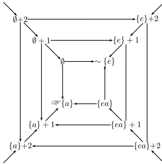
Figure 2: Candidate set 2 (a.k.a. search space, neighbourhood structure, topology) with insertion of third elements not present in the context into the reference set.
