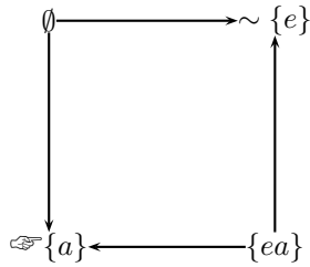
Figure 1: Candidate set 1 (a.k.a. search space, neighbourhood structure, topology) without insertion of third elements not present in the context into the reference set.
