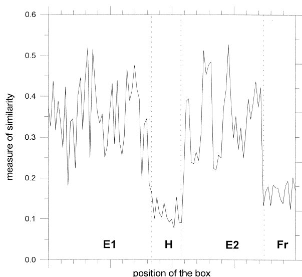
Fig. 1 The similarity between the content of a box of length m = 100 moving along the concatenation of texts in different languages, and an arbitrary English text. The concatenation consists of an about 8000 character long English text (E1), a 2640 character long Hungarian text (H), another English text (E2) that is 6450 characters long, and a 2860 character long French text (Fr). The multiplying vector was constructed from a different English text. A deep “valley” can be observed starting at the point where the end of the box is penetrating into the non-English texts, i.e. m characters before the non-English texts. The x axis represents the place of the beginning of the box, and the valley lasts until the box contains any part of this text. These valleys differ significantly enough to split the symbol sequence to sub-sequences according to similarity, meaning the same language in our case. ( n = 3 for all vectors.)
